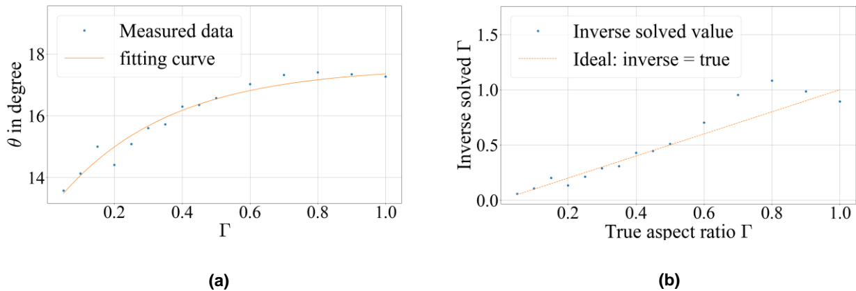
Figure 1. Forward model fitting and inverse estimation of the disturbance aspect ratio based on the wake opening angle \theta . (a) Forward model fitting of \theta as a function of \Gamma . (b) Inverse estimation of \Gamma based on the measured wake angle \theta .
