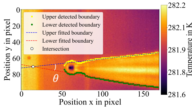
Figure 2. Thermographic wake structure with extracted wake boundaries and wake angle \theta .
